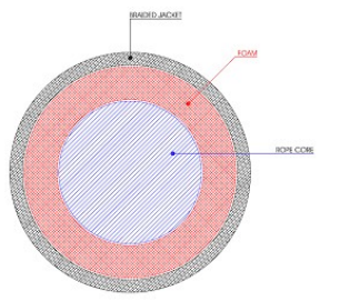
Cross-Sectional Diagram of Integral Flotation Buoyancy System
